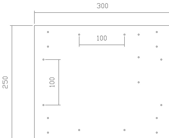
Bottom plate size and installation diagram
